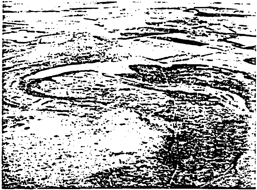
Figure 6.--Oblique aerial photograph of collapse features near Harroun, N. Mex. Some meanders of the Pecos River may have originated as similar semicircular features. View is toward the northwest; the Pecos River is in the background.
